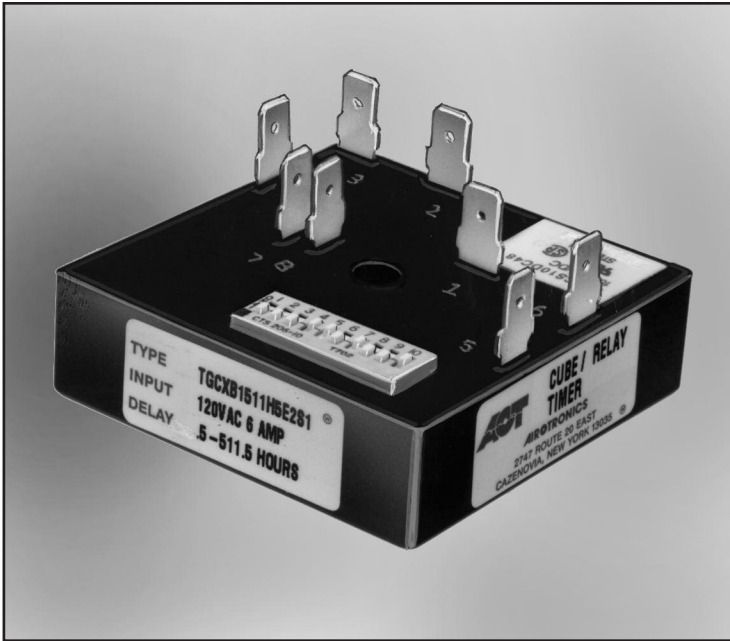
SWITCH SETTINGS 1, 2 & 6 ON = 17.5 HRS.
