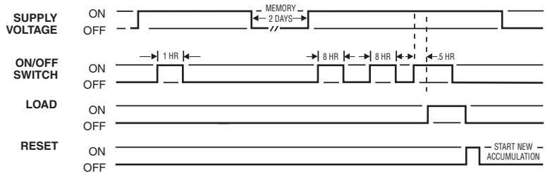
SWITCH SETTINGS 1, 2 & 6 ON = 17.5 HRS.
